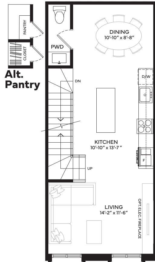
Main Level
